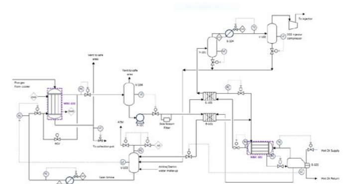
Figure 2: PETRONAS MBC Flue Gas Process Flow Diagram
